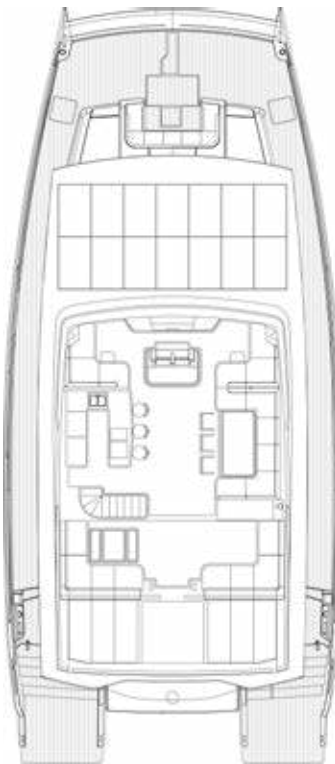
UPPER DECK 3-DECK OPEN Alternative saloon layout
