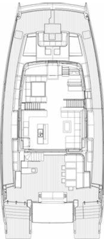
MAIN DECK 3-DECK Alternative saloon layout
